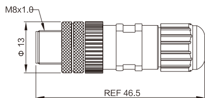
M8公头/Male molded cable
