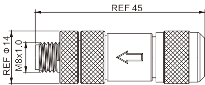
M8公头/Male molded cable
