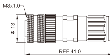
M8母头/Female molded cable
