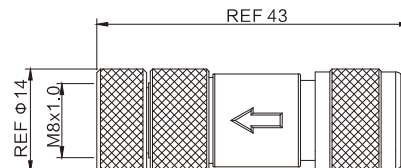
M8母头/Female molded cable
