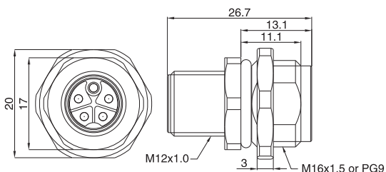
M12公头/Male Panel mount
