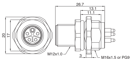
M12公头/Male Panel mount
