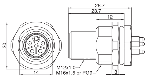
M12公头/Male Panel mount
