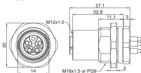
M12母头/Female Panel mount
