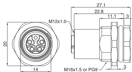
M12母头/Female Panel mount
