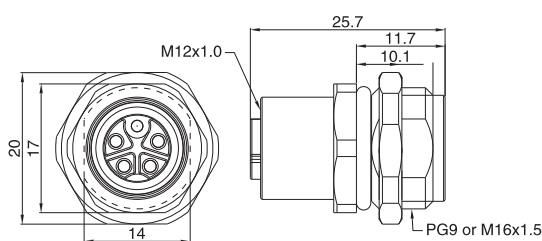
M12母头/Female Panel mount
