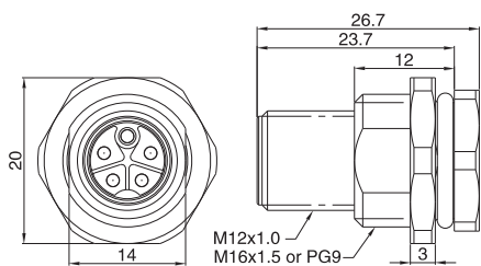
M12公头/Male Panel mount
