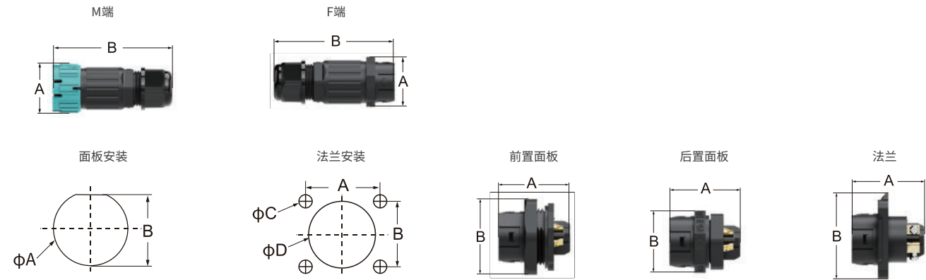
连接器机械尺寸 Mechanical dimensions of the connector
